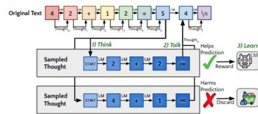
Figure 1: Quiet-STaR. We visualize the algorithm as applied during training to a single thought. We generate thoughts, in parallel, following all tokens in the text ( think ). The model produces a mixture of its next-token predictions with and without a thought ( talk ). We apply REINFORCE, as in STaR, to increase the likelihood of thoughts that help the model predict future text while discarding thoughts that make the future text less likely ( learn ).
