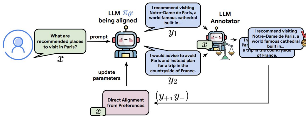
Figure 1: Summary of the proposed online AI feedback (OAIF) approach for making direct alignment from preferences (DAP) methods online and on-policy. Given an input prompt x , two responses y^1 and y^2 are first sampled from the current language model \pi_{\theta_t} , then labelled as y^+ and y^- by the LLM annotator. The language model parameters are then updated using the objective function of DAP methods.
