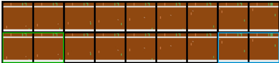
Figure 4: Pixel perfect predictions in Pong . The top row displays a test trajectory collected in the real environment. The bottom row depicts the reenactment of that trajectory inside the world model. More precisely, we condition the world model with the first two frames of the true sequence, in green. We then sequentially feed it the true actions and let it imagine the subsequent frames. After only 120 games of training, the world model perfectly simulates the ball’s trajectory and players’ movements. Notably, it also captures the game mechanic of updating the scoreboard after winning an exchange, as shown in the blue box.
