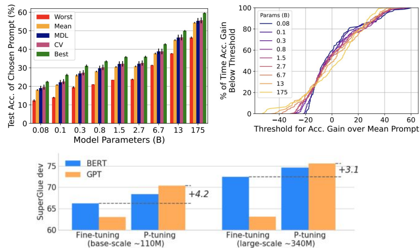
Figure 1. Average scores on 7 dev datasets of SuperGlue. GPTs can be better than similar-sized BERTs on NLU with P-tuning.
