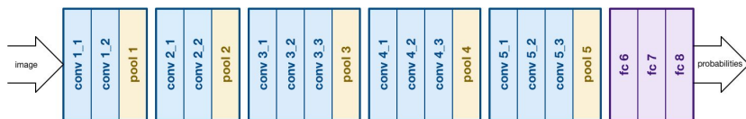
VGGNet architecture (2014)
