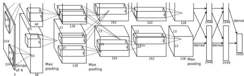
AlexNet architecture (2013)
