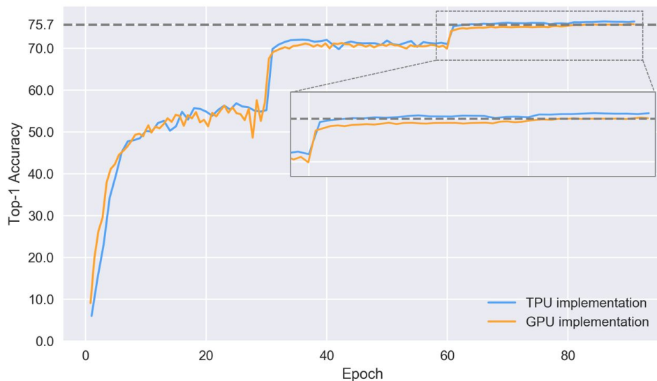
Top-1 accuracy learning rate of TPU vs GPU on ImageNet
