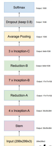
Inception v4 (2016)
