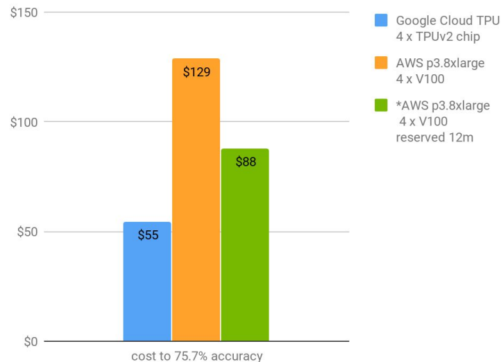
Cloud cost to reach 75.7% top-1 accuracy
