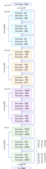
ResNet (2015)
